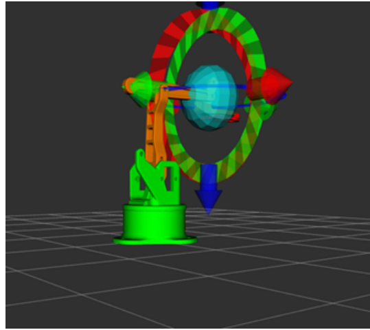
Fig. 1. URDF model of Manipulator Robot in RVIZ
